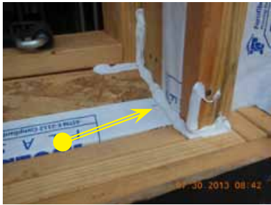
4. Sealant applied as shown
